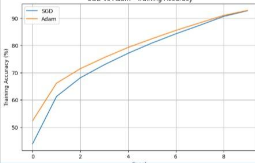
SGD vs Adam - Training Accuracy
